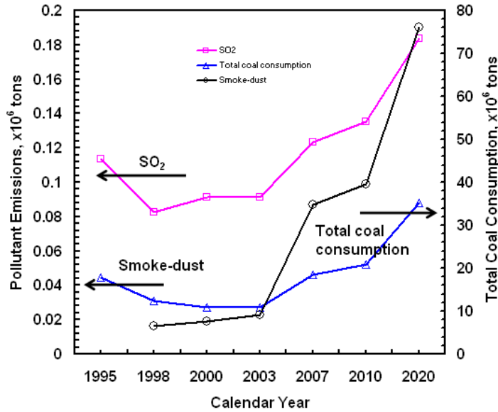
Figure 1 Trends of major pollutant emission level and total coal consumption in Huainan.
