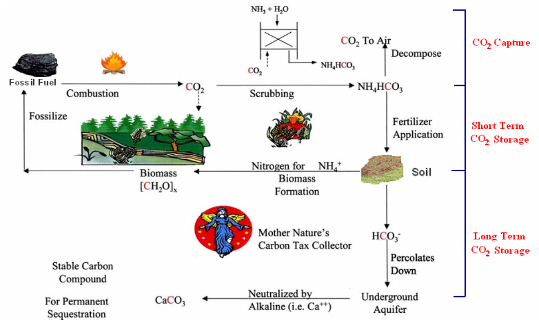
Figure 4. A schematic of three stages of sequestering CO 2 by the ecosystem
