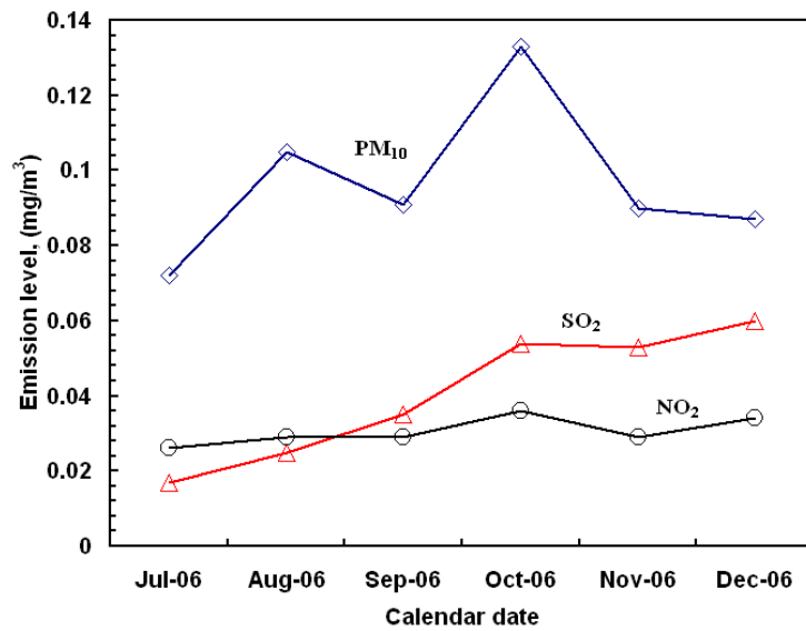
Figure 2. Measured emission levels of SO 2 , NO 2 and PM in 2006 in Huainan.
